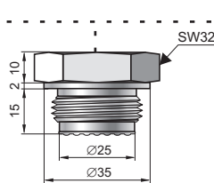
CM30×2 type M30×2 with flush diaphragm
